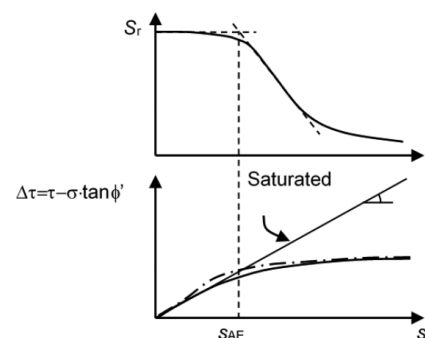
Fig. 4. Contribution of suction to shear strength (source [19])
